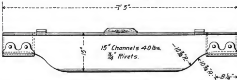
Figs. 4426-4128. Twin Channel Truck Bolster. Vanderbilt Patent.
